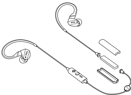
Lithium-Polymer-Akku (0,37 Wh)
