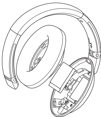
Lithium-Polymer-Akku (2,22 Wh)
