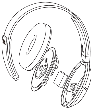
Litium-polymer-batteri (0,37 Wh)
